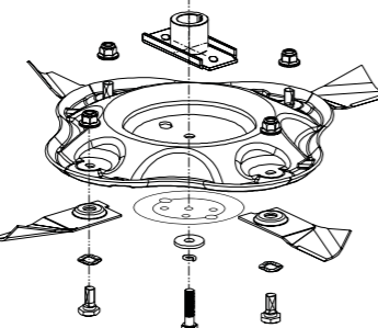
Cuchilla "Quadcut"
