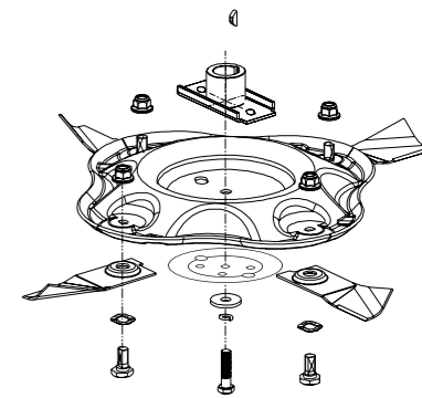
Quadcut® Blade
