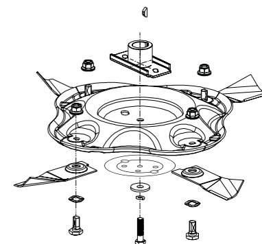
Lame Quadcut®
