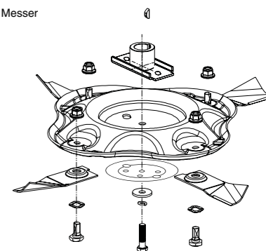
Quadcut® Messer
