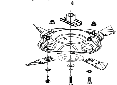
Lama Quadcut®
